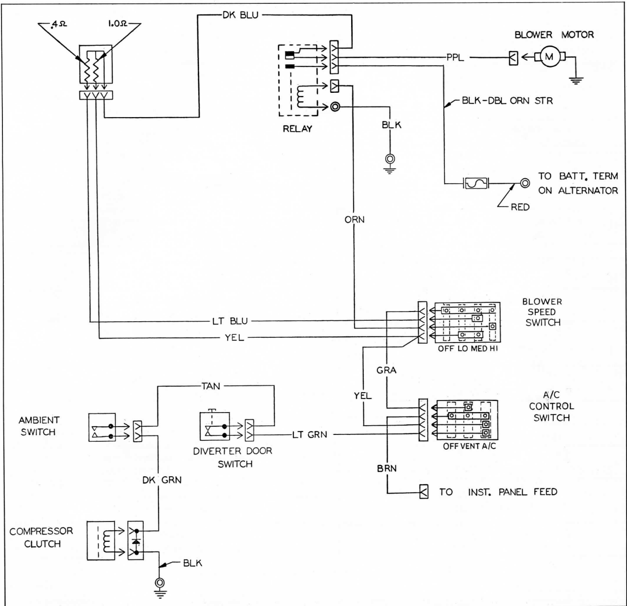
Fig. 1A-33 Electrical Schematic—Firebird
